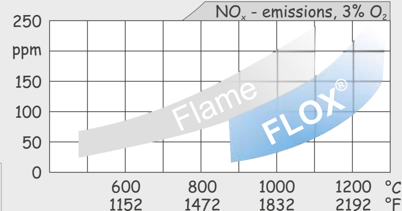
Exhaust gas temp. at the recuperator entry
